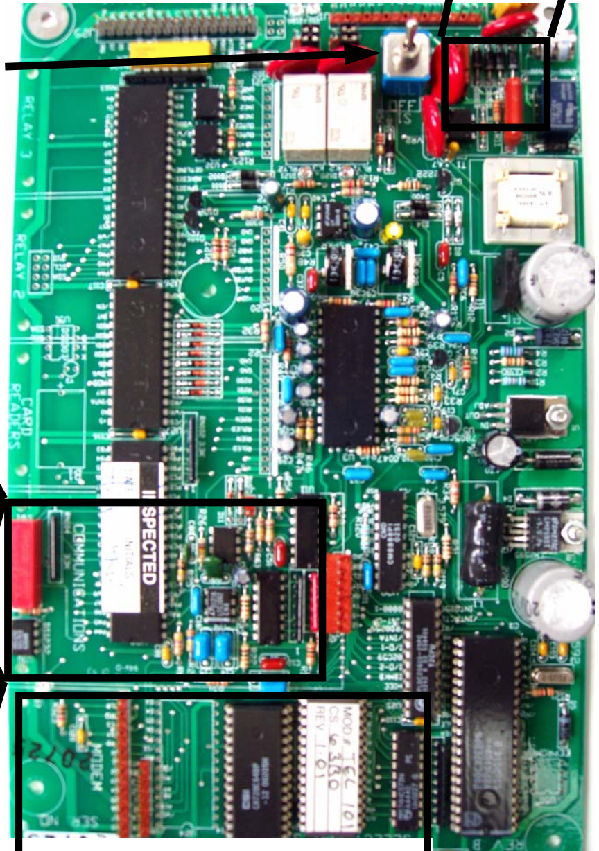
MAIN BOARD
